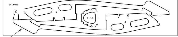
1/8" X 5-1/8" X 23-3/4" PLY FUSELAGE DOUBLERS
