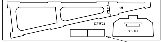
1/8" X 5-3/4" X 17-3/4" PLY TANK HATCH DOUBLERS
