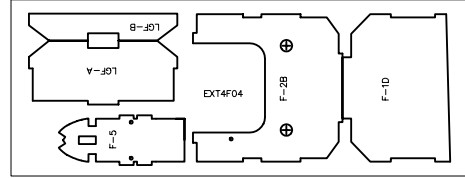
1/8" X 5-3/4" X 15" PLY
